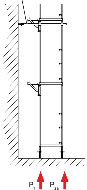
Scaffold retainer
