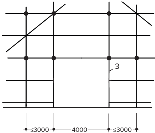
Bridged bay 400
