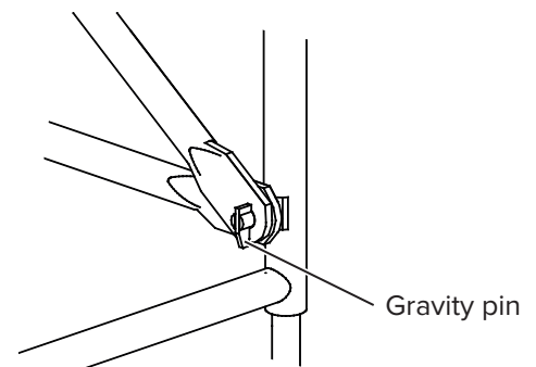
Attachment of diagonal at bottom
