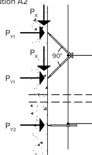
Tying solution A2
