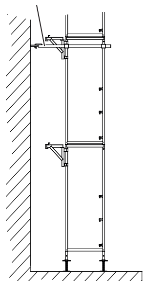
Scaffold retainer
