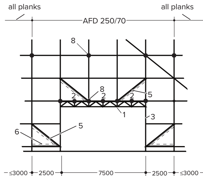
Bridged bay 700
