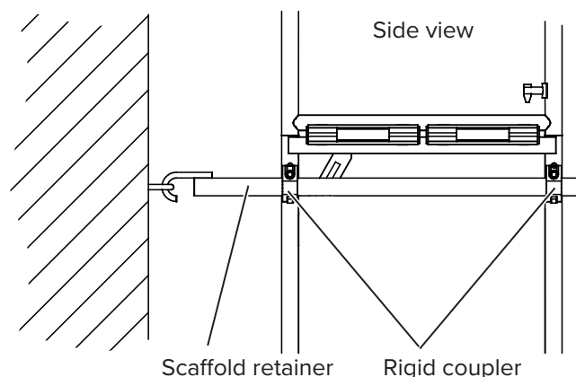
Tying solution A1: Long scaffold retainer
