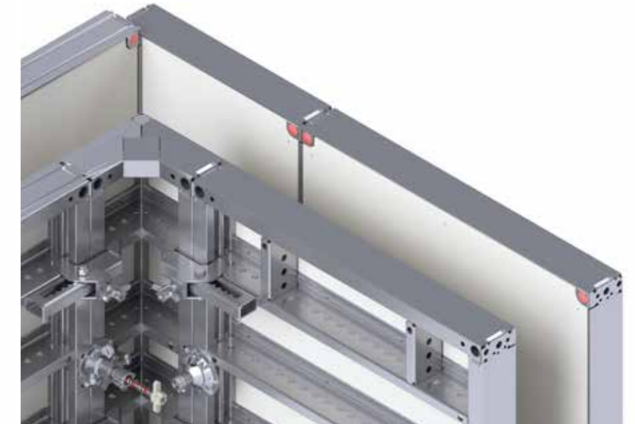
► Detailed view of the corner. The one-sided PLATINUM 100 tie is easily visible, as is the bracket for the crane hook
